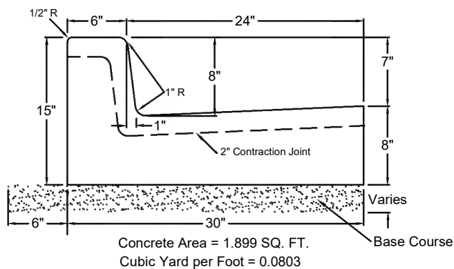
Type B - 30" ADA Access
