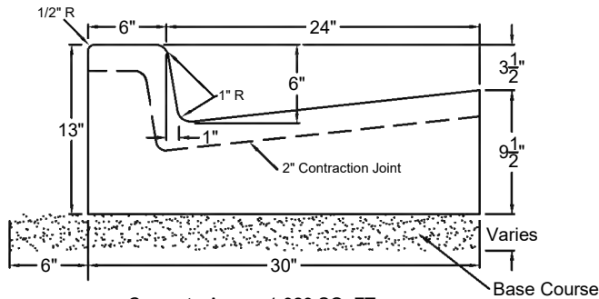
Type A - 30" Standard
