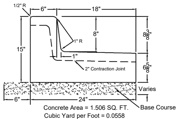
Type B - 24" Reverse Pan
