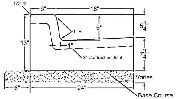
Type A - 24" ADA Access
