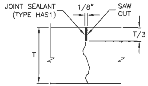
STRESS CUT DETAIL 2
