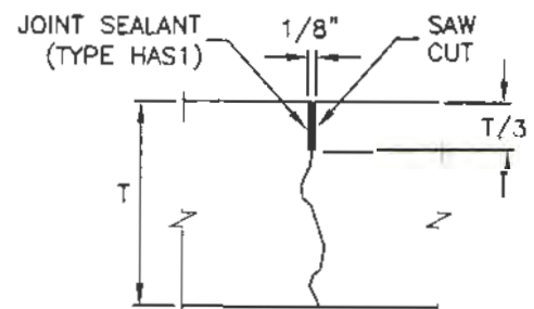
STRESS CUT DETAIL 2
