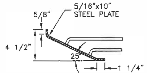
FACE PLATE DETAIL
