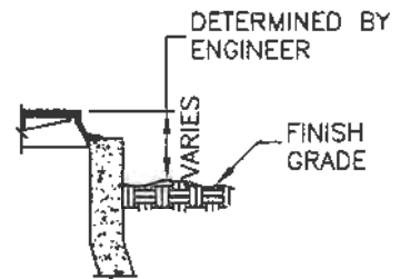
DETAIL (UNIMPROVED AREAS)
