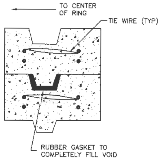
GASKET DETAIL
