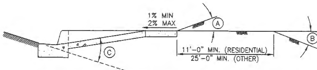
SECTION A-A APPROACH REQUIRING SERVICE TRUCK ACCESS
