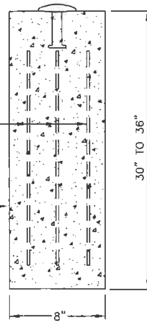
SECTION OF BASE TYPICAL SETTING
