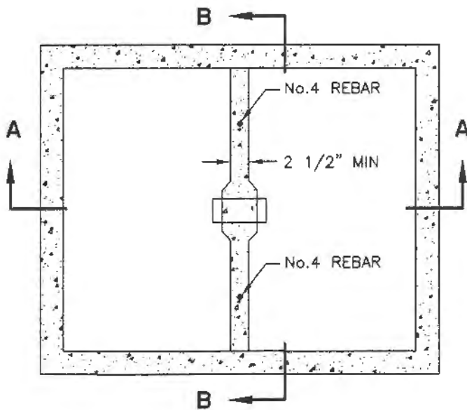
BOX PLAN
