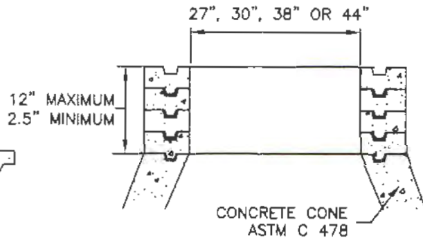
CONE SECTION
