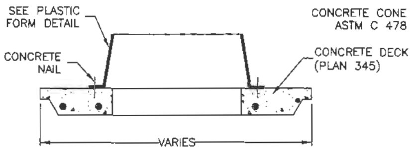
DECK SECTION
