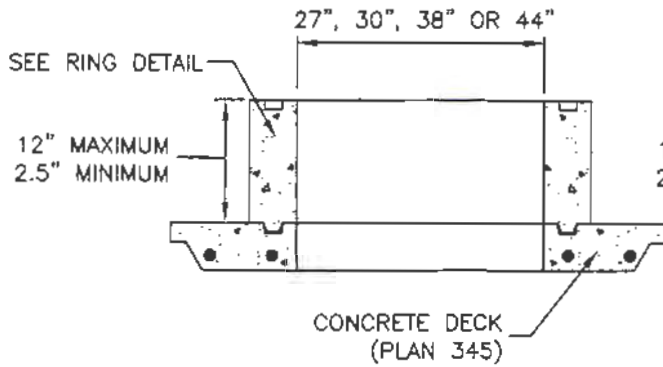
DECK SECTION
