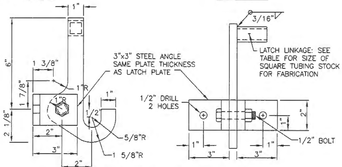
LEFT LATCH DETAIL (TYPICAL)
