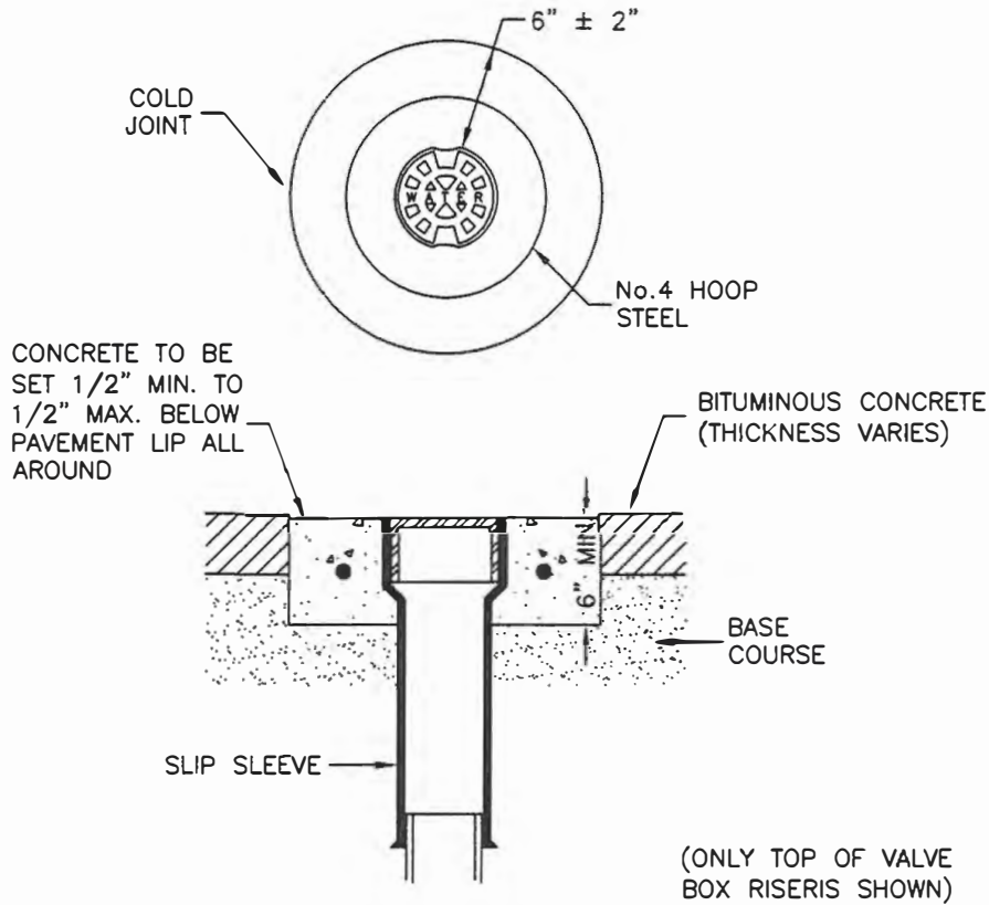
BITUMINOUS PAVEMENT
