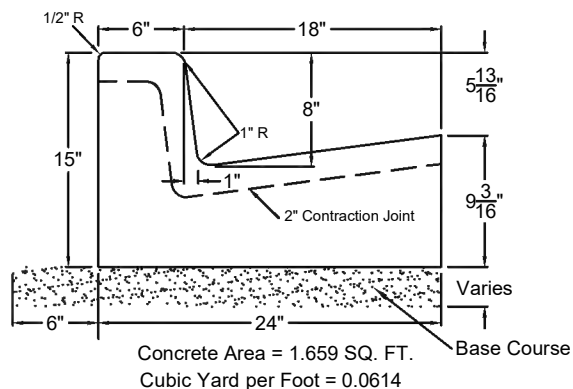
Type B - 24" Standard
