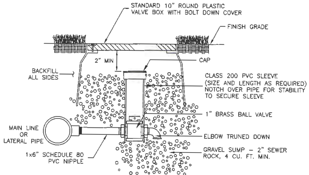
TYPE A - MANUAL DRAIN VALVE
