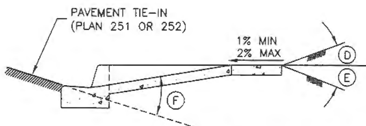
SECTION A-A TYPICAL DRIVEWAY APPROACH
