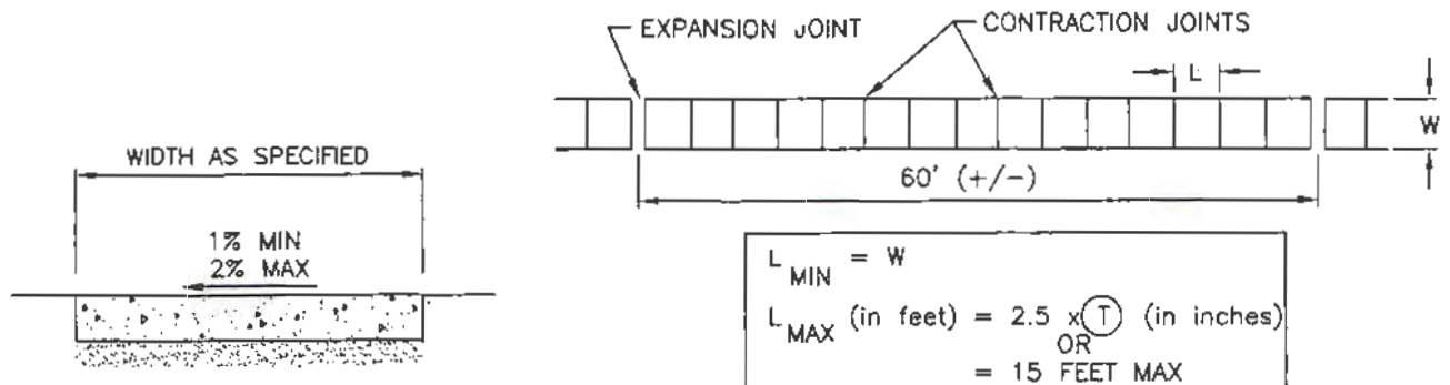
SIDEWALK JOINT DETAIL
