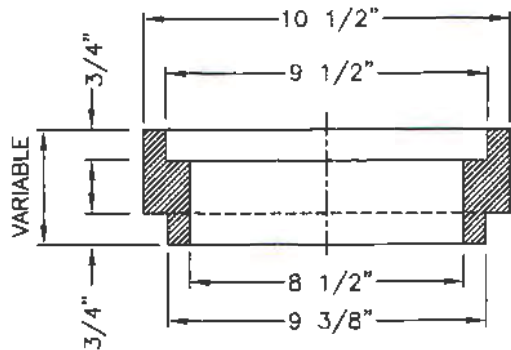
EXTENSION
