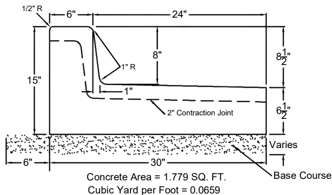
Type B - 30" Reverse Pan
