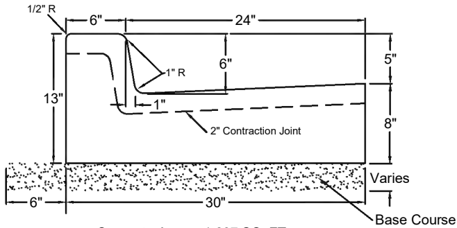
Type A - 30" ADA Access
