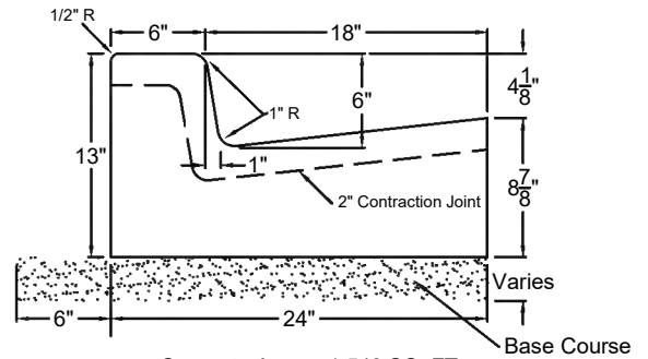
Type A - 24" Standard
