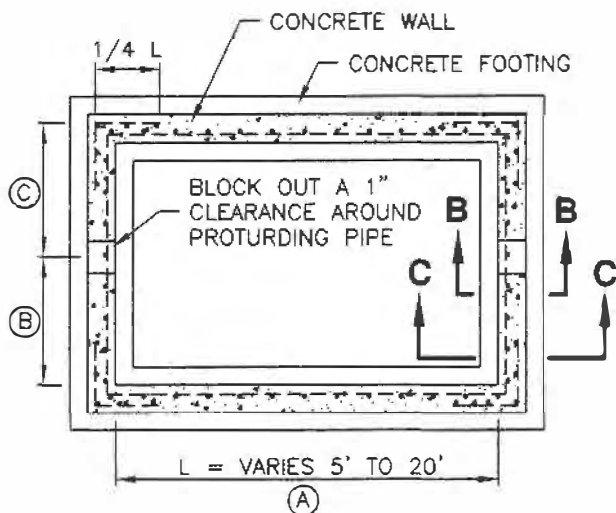
BOX PLAN
