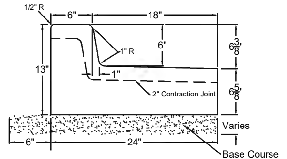
Type A - 24" Reverse Pan
