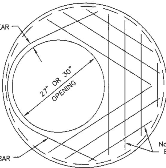
60" DECK PLAN
