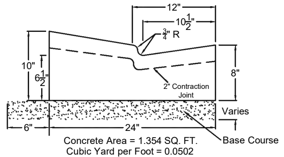
Type H - 24" Standard
