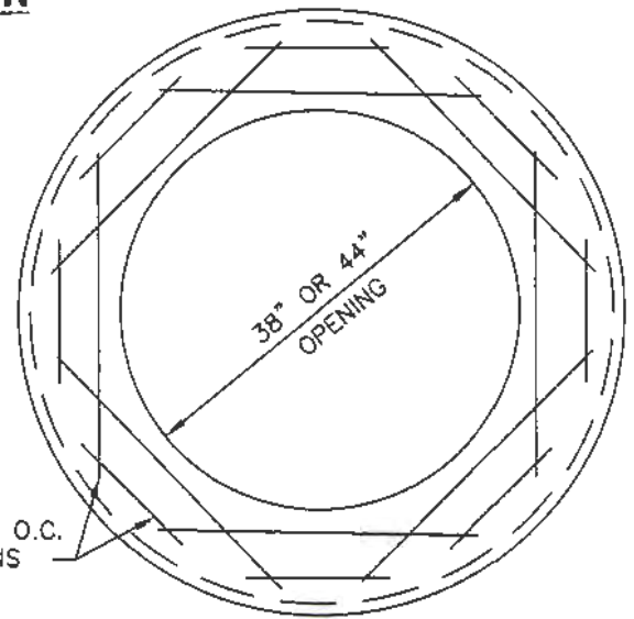
60" DECK PLAN
