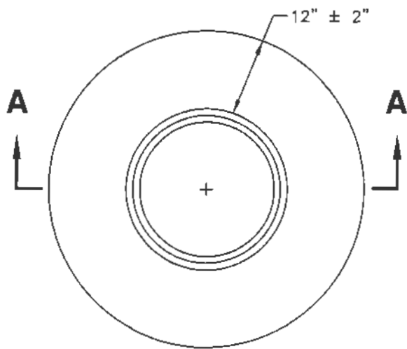
PLAN (ROUND FRAME)
