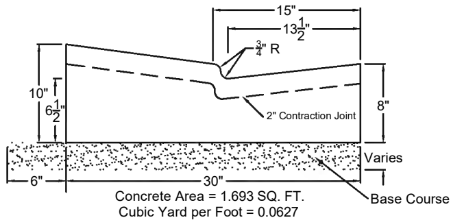
Type H - 30" Standard
