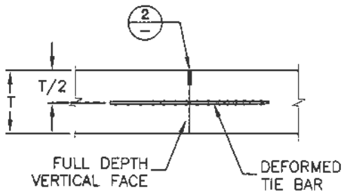
T-2 VERTICAL FACE
