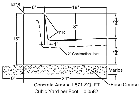
Type B - 24" ADA Access
