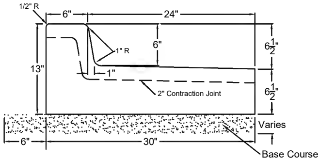
Type A - 30" Reverse Pan
